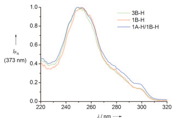
Figure 5. Normalized excitation spectra of ONs 1B-H and 3B-H and duplex 1A-H/1B-H, monitoring emission intensity at 373 nm ( c=1.2 \mu\text{M} ON in 10 mM \text{NaH}_2\text{PO}_4 , 0.15 M NaCl, pH 7.0, T=20^\circ\text{C} ). I_f =fluorescence intensity.
