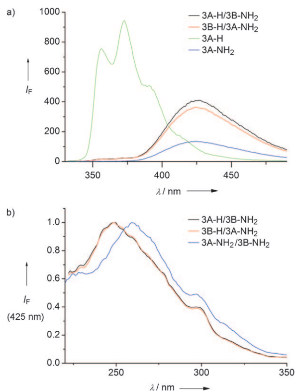
Figure 8. a) Fluorescence emission spectra of the triple-modified duplexes with homo and hetero phenH and phenNH 2 pairs and the corresponding single strands. Excitation wavelength: 252 nm; b) normalized excitation spectra monitoring emission at 425 nm. Conditions: T = 20 °C, c = 1.2 μM duplex in 10 mM NaH 2 PO 4 , 0.15 M NaCl, pH 7.0. I f = fluorescence intensity.
