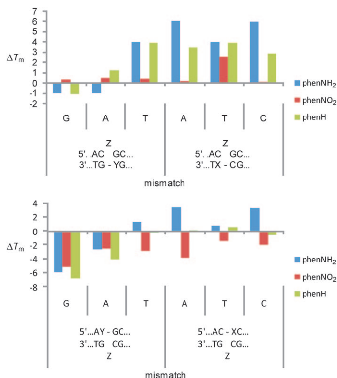
Figure 4. \Delta T_m data from UV melting curves (conditions as in Table 2) from mismatched duplexes with and without a phenR residue (Z) in the bulge position next to the mismatch. The phenR-containing strands are from the mono-series strand A (top) and strand B (bottom) that were paired to their mismatched DNA complement.
