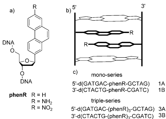
Figure 1. a) Structure of the phenanthrenyl- C -nucleoside units; b) cartoon representation of the expected zipper-like duplex structure; c) sequence information of the mono- and triple-modified duplexes. A and B refer to strand A and B, respectively, whereas 1 and 3 designates single or triple modification, respectively. phenR denotes the ensemble of phenH, phenNH 2 , or phenNO 2 residues.
