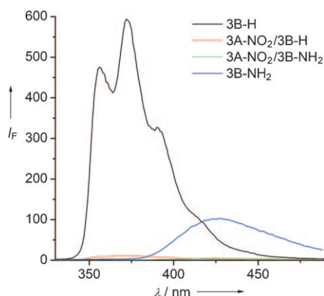
Figure 7. Quenching of phenH and phenNH 2 fluorescence in the triple series upon pairing with a complementary ON containing three PhenNO 2 residues. Excitation wavelength: 252 nm (for phen-H) or 264 nm (for phenNH 2 ), c = 1.2 μM duplex in 10 mM NaH 2 PO 4 , 0.15 M NaCl, pH 7.0, T = 20 °C. I f = fluorescence intensity.
