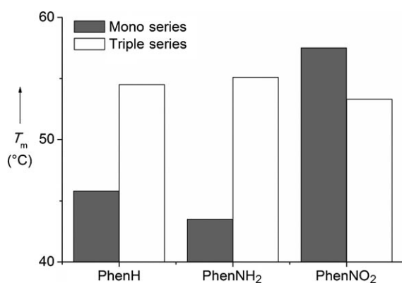
Figure 3. Comparison of T_m data for homo mono- and triple-modified duplexes.
