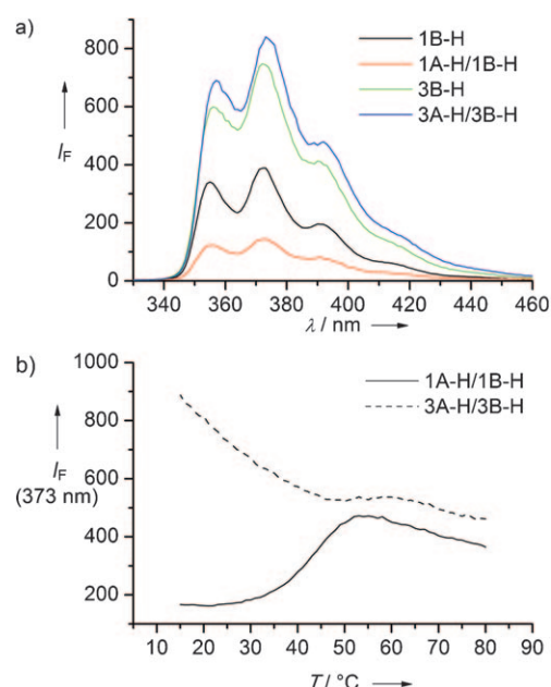
Figure 6. a) Fluorescence spectra of phenH-containing ONs and duplexes. b) Melting curves of the duplexes 1A-H/1B-H and 3A-H/3B-H as monitored by the emission intensity at 373 nm. Conditions: excitation wavelength 252 nm; c=1.2 \mu\text{M} duplex in 10 mM \text{NaH}_2\text{PO}_4 , 0.15 M NaCl, pH 7.0; T=20^\circ\text{C} (for a)); heating rate 0.5^\circ\text{C} per min (for b)). I_f =fluorescence intensity.
