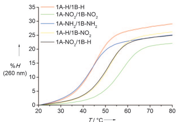
Figure 2. UV melting curves (260 nm) of selected phenR-containing duplexes of the mono series. c = 1.2 μM in 10 mM NaH 2 PO 4 , 0.15 M NaCl, pH 7.0.
