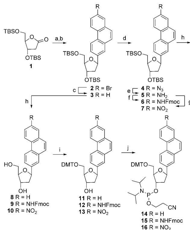
Scheme 1. Reagents and conditions: a) 2,7-dibromophenanthrene, n BuLi (1.1 equiv), THF, –78°C, 1 h, then 1 (1 equiv) in THF, –78°C, 4 h; b) Et 3 SiH (3 equiv), BF 3 ·OEt 2 (3 equiv), CH 2 Cl 2 , –78°C, 6 h. Yields: 2 (15%), 3 (1.5%); c) n BuLi (1.1 equiv), THF, –78°C, 1 h, then H 2 O. Yield: quantitative; d) n BuLi (1 equiv), THF, –78°C, 40 min, TsN 3 (1.2 equiv), THF, –70°C, 5 h, Na 2 HPO 4 (2 equiv), H 2 O, Et 2 O, THF, +5°C, 12 h. Yield: 91%; e) SnCl 2 , MeOH, THF, 0°C → RT, 1.5 h. Yield: 85%; f) FmocCl (2 equiv), i Pr 2 NEt (2 equiv), CH 2 Cl 2 , RT, 5 h. Yield: 77%; g) dimethyl dioxirane (0.075 M, 4.1 equiv), acetone, MeCN, –80°C, 2 h. Yield: 75%; h) TBAF (1.4 equiv), THF, RT or (HF) 3 NEt 3 (8 equiv), THF, RT, 24 h. Yield: 75–95%; i) 4,4'-dimethoxytrityl (DMT) chloride (1.2–1.9 equiv), pyridine, 0°C, 5 h. Yield: 73–87%; j) ( i Pr 2 N)(NCCH 2 CH 2 O)PCl (1.5 equiv), i Pr 2 NEt (3 equiv), THF, RT, 1.5 h. Yield: 70–83%. Fmoc = 9-fluorenylmethoxycarbonyl, TBAF = tetra- n -butylammonium fluoride, TBS = tert -butyldimethylsilyl.
